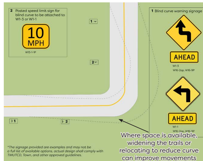
FIGURE 5.3: TYPICAL BLIND CURVE DESIGN
