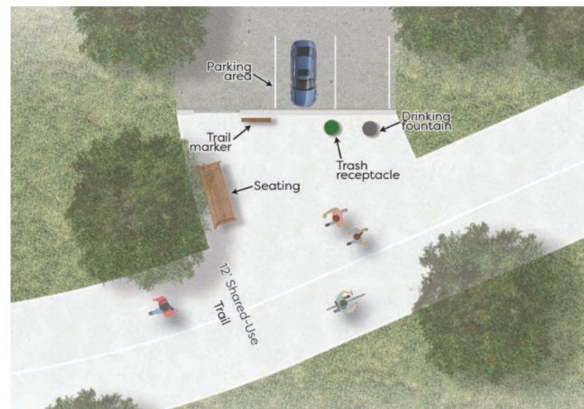
FIGURE 5.12: EXAMPLE MINOR TRAILHEAD
